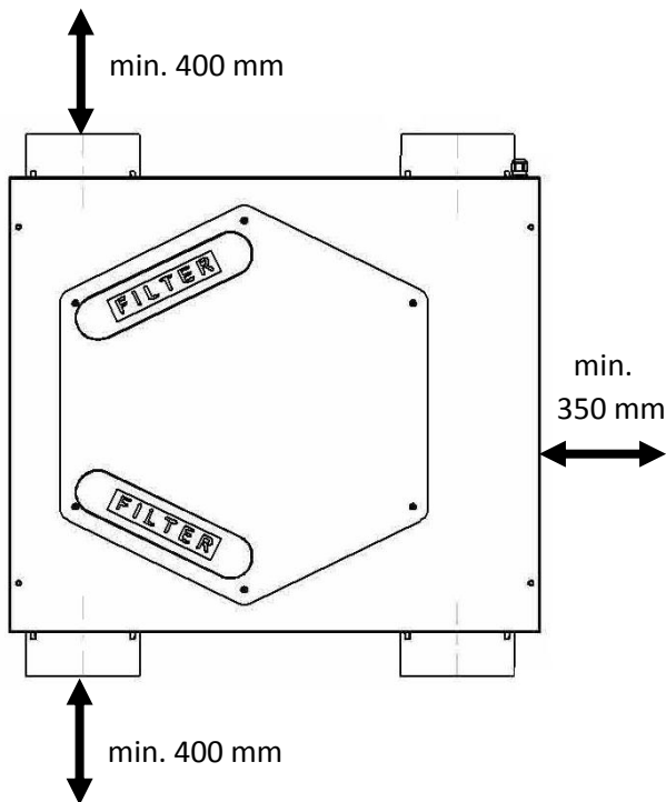
HRV 20 Wandmontage
