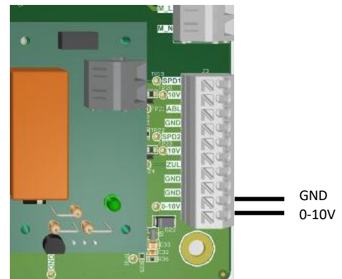
HRV 30 / HRV 35
